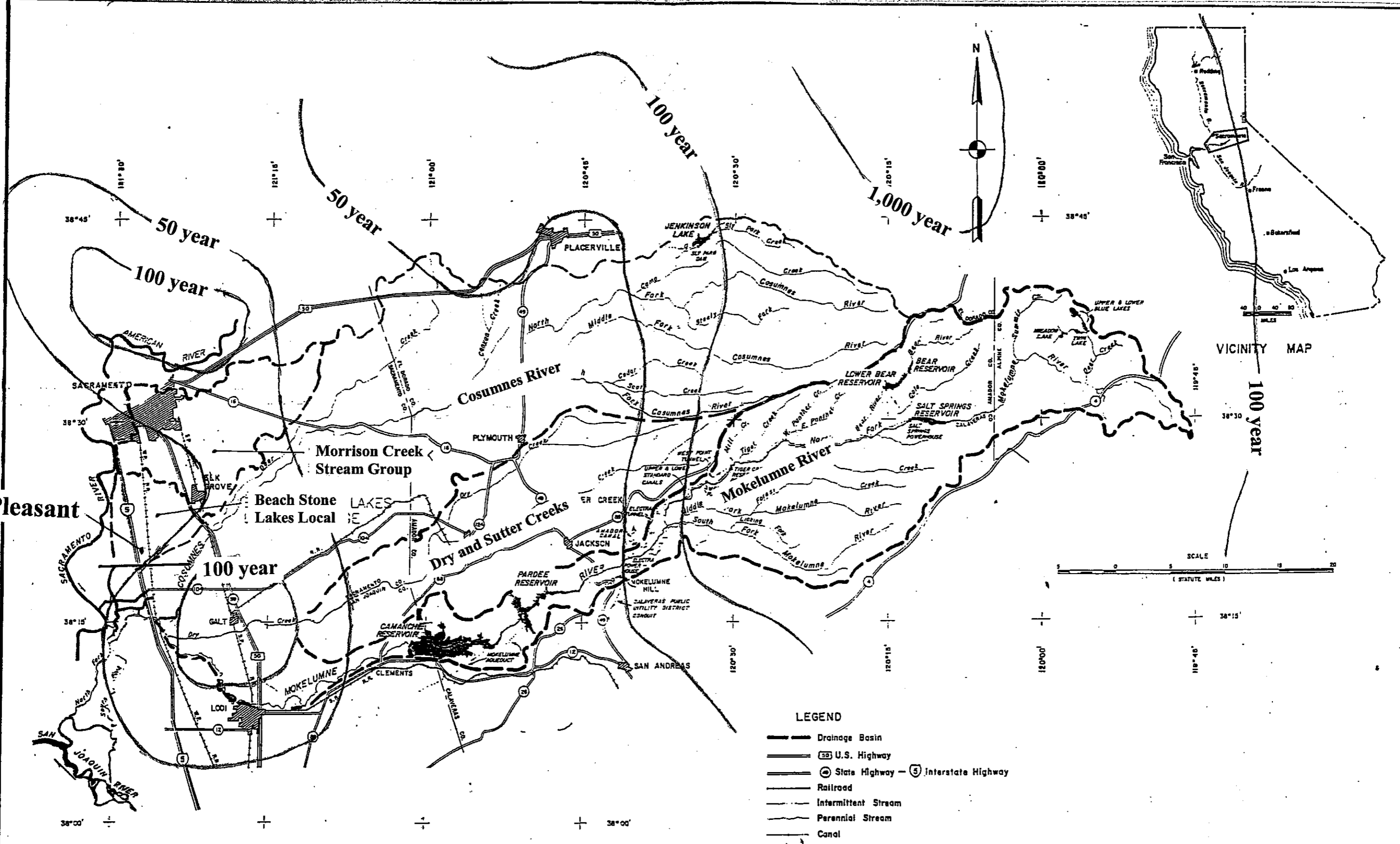
Storm of February 11 to 20, 1986 Return Period for Total Storm Depth
